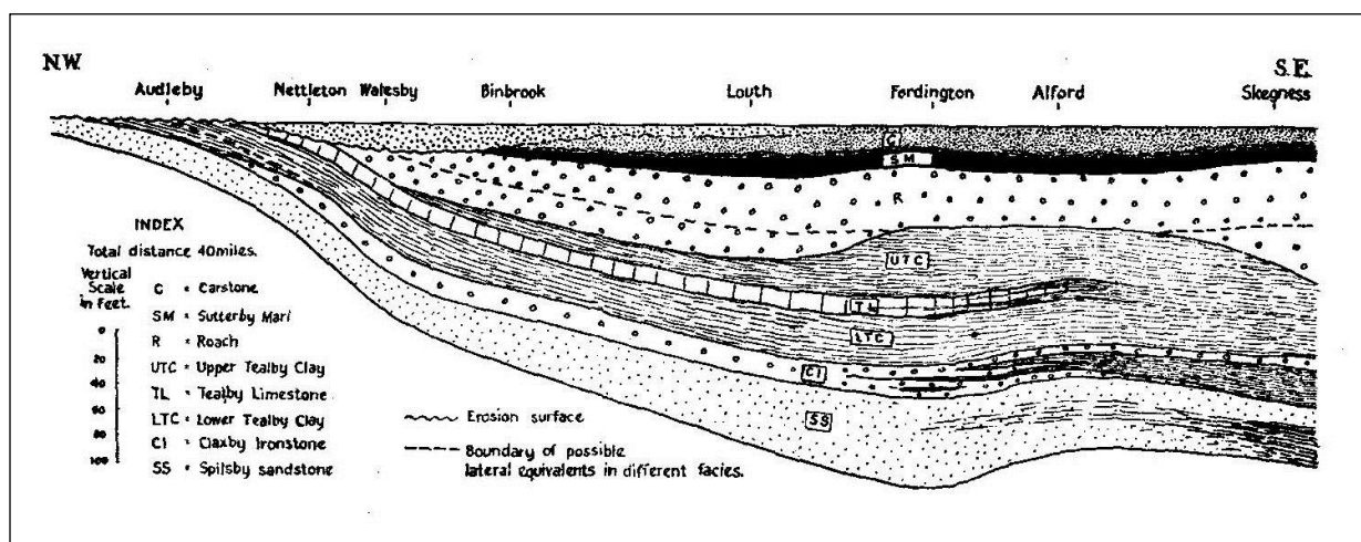
Figure 7: Diagrammatic section showing relationships of the subdivisions of the Lower Cretaceous rocks 10 .
