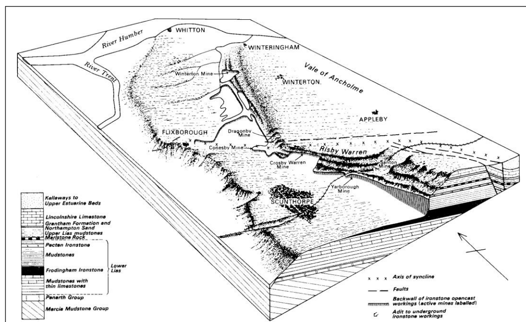
Figure 5: Block diagram of the Scunthorpe area showing the Frodingham Ironstone workings 9 .
